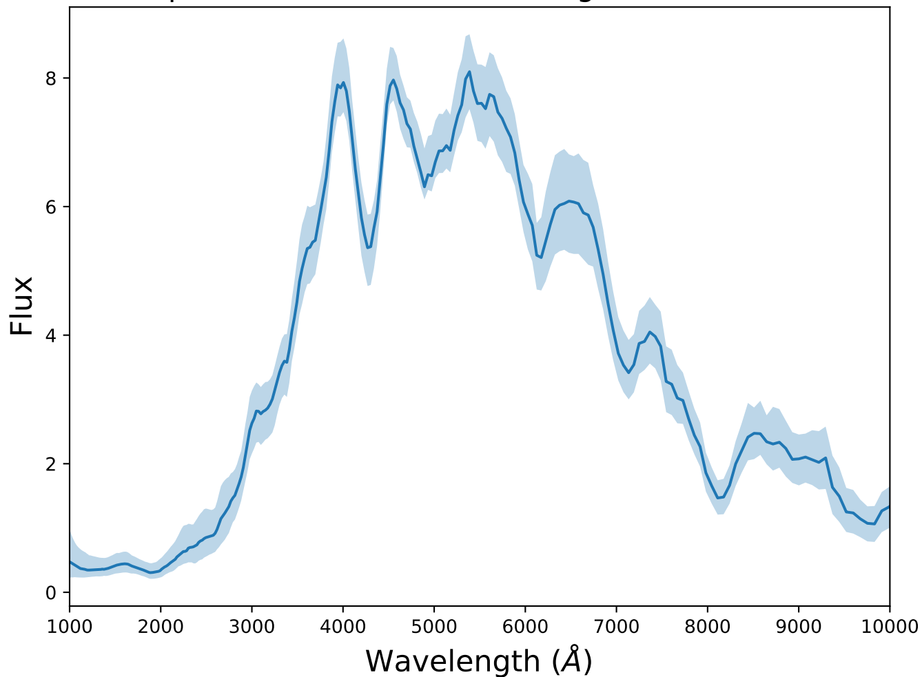
Spectrum 5 for transient 91bg-like at z=1.35
